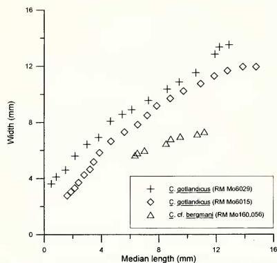
TEXT-FIG. 6. Median length-width graphs for individual intermediate sclerites of Chelodes gottlandicus (RM Mo6029 and Mo6015) and C. cf. bergmani (RM Mo160.056).
